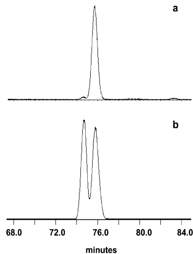
Figure 3. Chiral GC–MS chromatogram for 3 isolated from the (a) V-BrPO-catalyzed reaction and the (b) TBCO reaction with 1 . The retention time for the single diastereomer of 3 isolated from V-BrPO reactions was 75.7 min. Diastereomers isolated from TBCO reactions eluted with retention times of 74.1 and 75.7 min, respectively. Gas chromatography was performed using 90 min, 155 °C isotherm runs.
